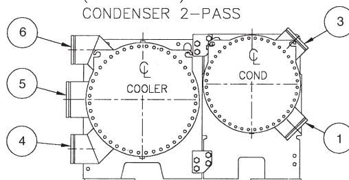
COMPRESSOR END
